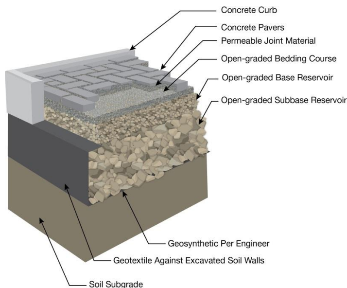
Figure 5.4-3. Full Infiltration Section Cross Section Source: Courtesy of ICPI
