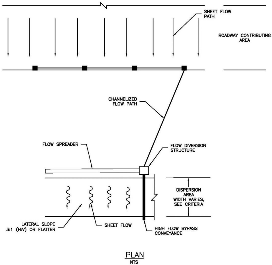
Figure 5.5-4. Channelized Dispersion Plan View
