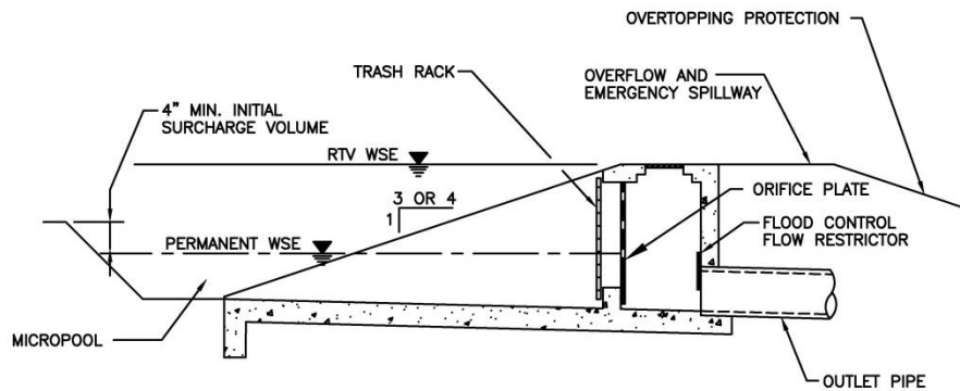
Figure 5.7-5. Example Orifice Plate Outlet Structure (Runoff Treatment Volume Only) Source: Adapted from UDFCD (48) 1
