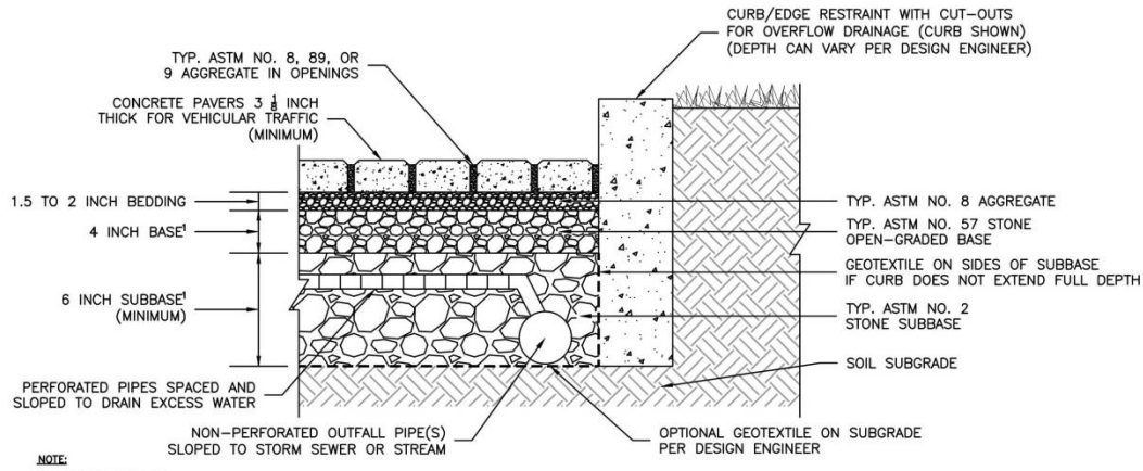
PARTIAL INFILTRATION NTS
